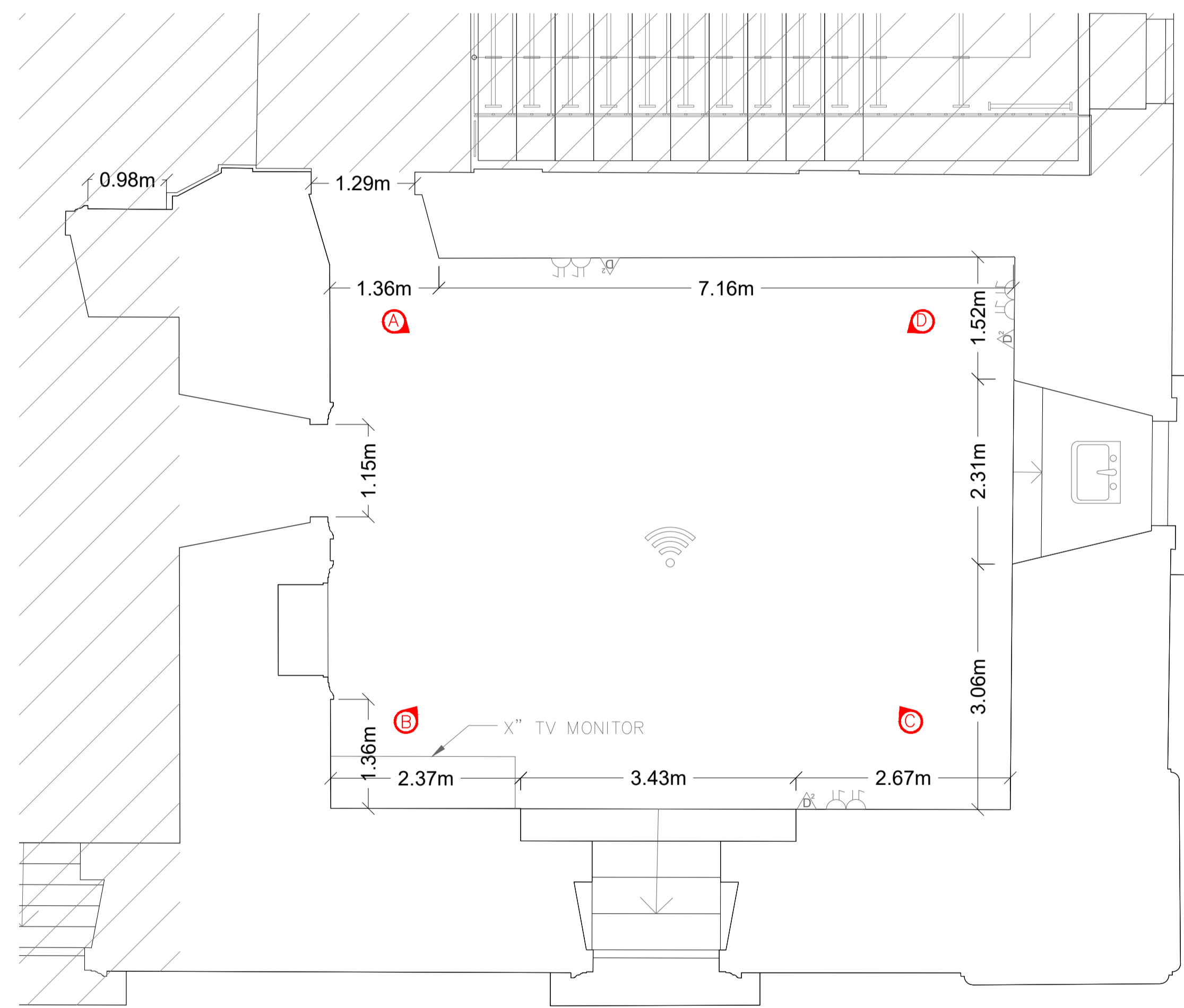
COMMUNITY SPACE SCALE 1:100
